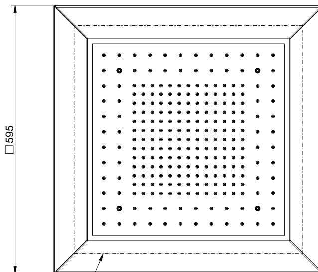
INSTALLATION MODE 2
