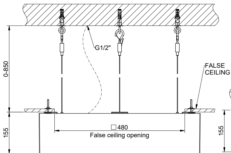
INSTALLATION MODE 1
