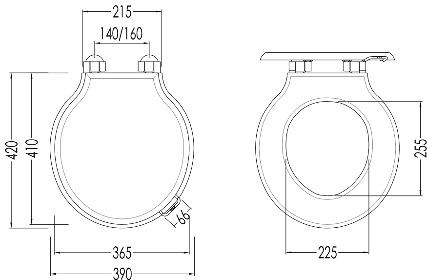
2. SEDILE LISTRATO MDF (cerniera soft-close) MDF SEAT (soft-close hinge)
