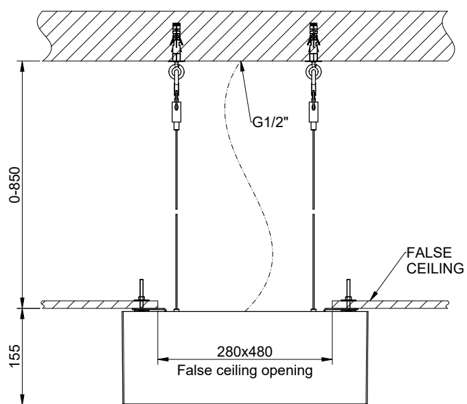
INSTALLATION MODE 1
